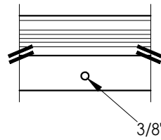
ASTRAGAL BOLT DETAIL OUTSWING THRESHOLD
