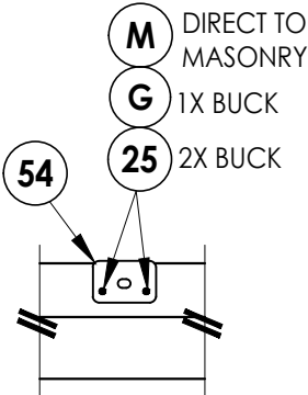
ASTRAGAL BOLT DETAIL STRIKE PLATE @ HEAD
