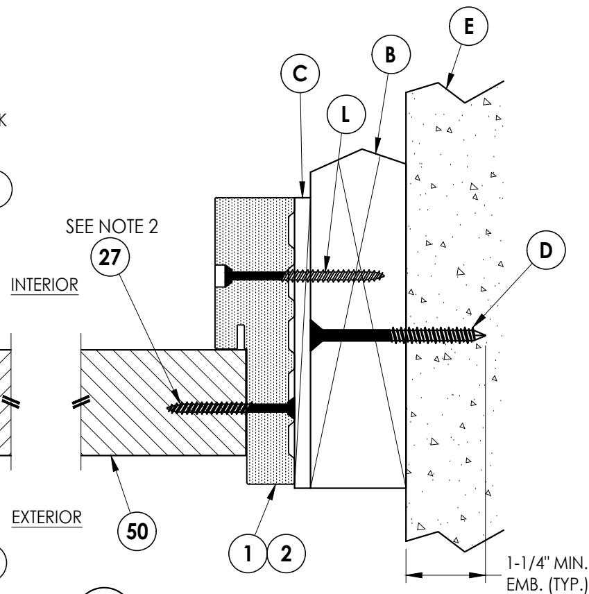
2 HORIZONTAL CROSS SECTION 6 Outswing Shown (Inswing Similar) Shown w/ 2X Buck
