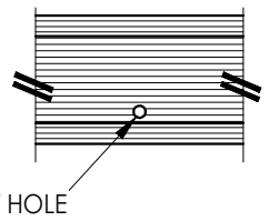
ASTRAGAL BOLT DETAIL ADA THRESHOLD
