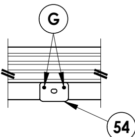
ASTRAGAL BOLT DETAIL INSWING THRESHOLD
